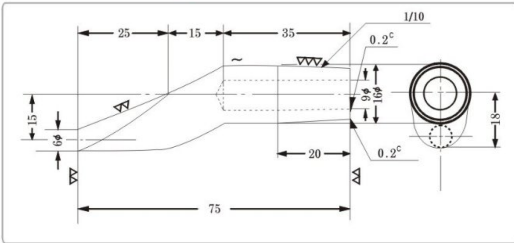
EK-C-1-2 小彎 One point bent
